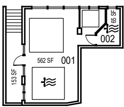
Basement Plan
